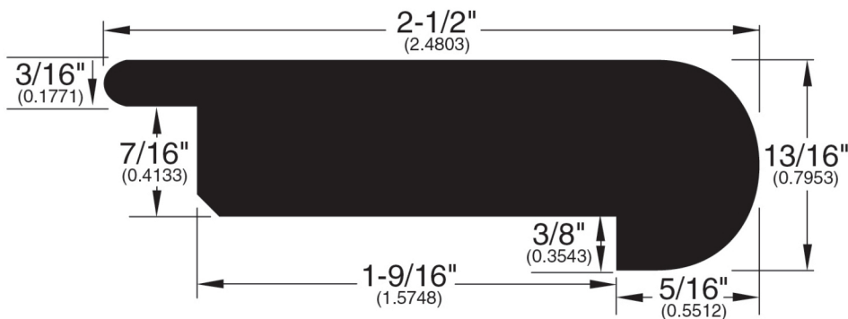
Stair Nose Overlap (131)
